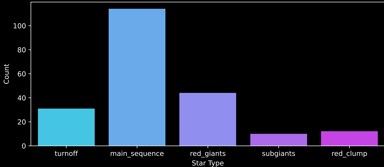
APOGEE DR17 Field: [135-30] Count plot of Star Type
