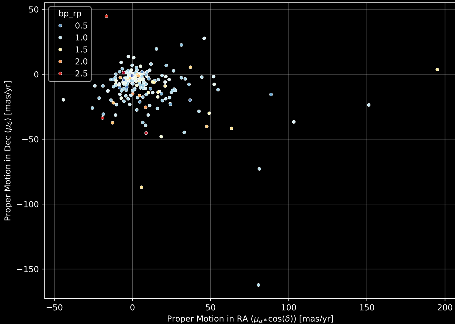
APOGEE DR17 Field: [135-30] Proper Motion Diagram (n= 211)
