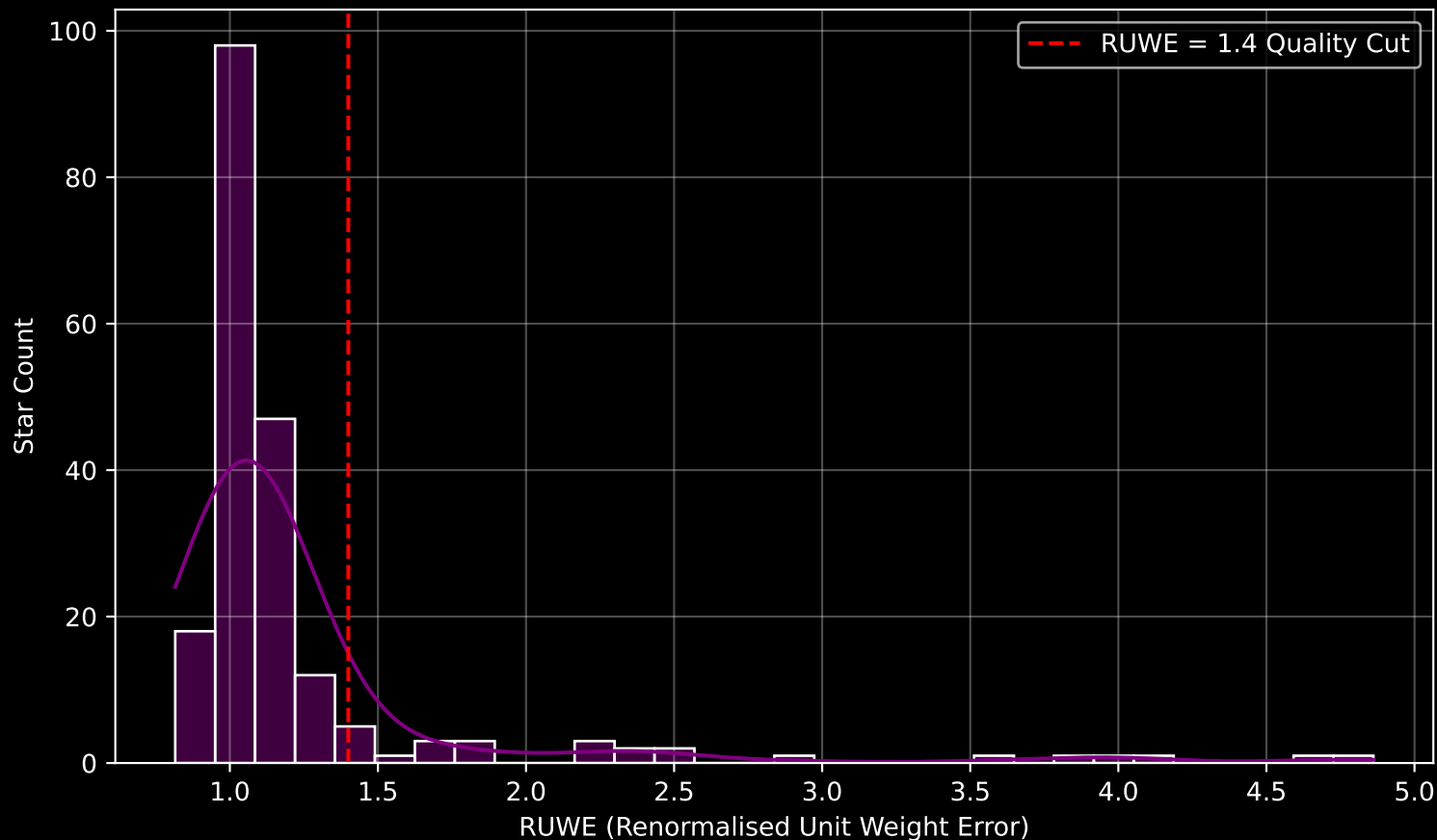
GAPOGEE DR17 Field [135-30] RUWE Distribution (n= 201)
