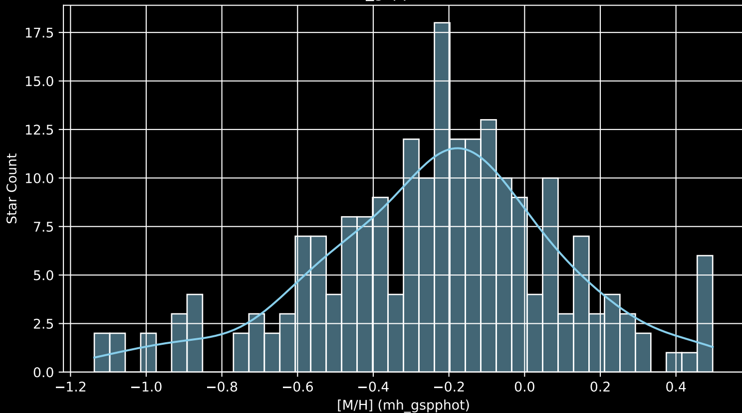
APOGEE DR17 Field: [135-30 [M/H] (mh_gspphot) (n= 210)
