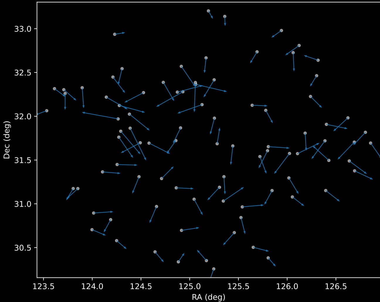
APOGEE DR17 Cluster 0 Proper Motion Vectors (n=88)
