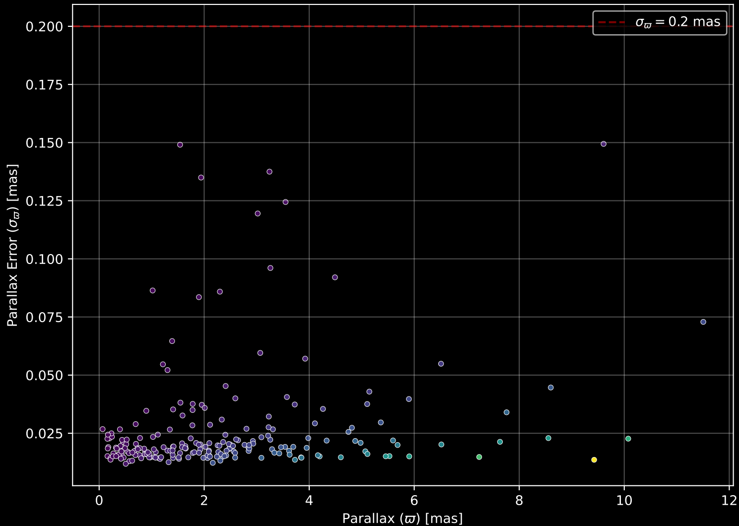
APOGEE DR17 Field: [135-30] Parallax Quality (n= 211)
